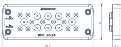
KES 20/24 10x Ø3.2 - 6.3mm 8x Ø5.5 - 10.5mm
